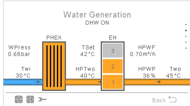
Water generation
