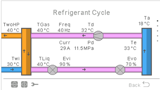
Refrigerant cycle
