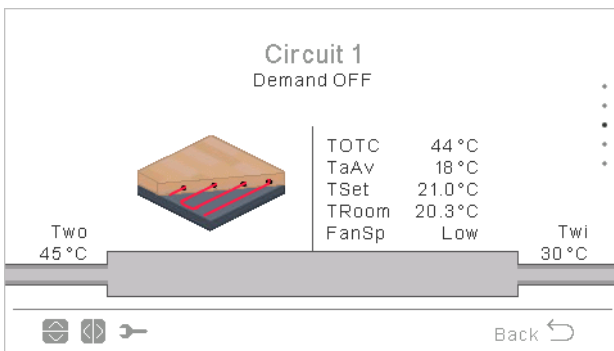
Circuit 1
